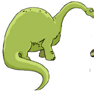
diplodocus
